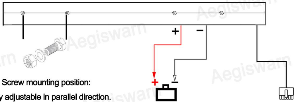
Auxiliary Battery
